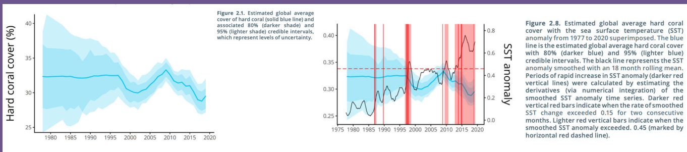
Figure 2. Declines of hard coral cover and correlation with sea surface temperature anomalies (GCRMN 2020)
